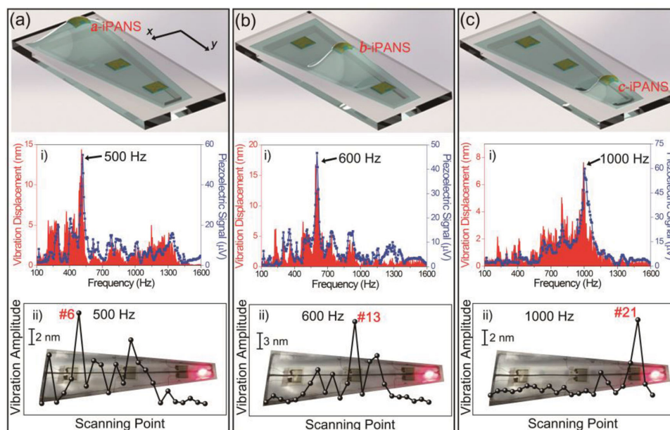
Figure 5. A vibration displacement and a piezoelectric signal generated by a,i) a-iPANS, b,i) b-iPANS and c,i) c-iPANS measured by LDV system and a sound level analyzer, respectively, in the frequency range of 100 Hz to 1600 Hz. A distribution of the vibration displacement and the piezoelectric signal were closely overlapped all over the frequency bandwidth. A single peak of vibration amplitude in response to a,ii) 500 Hz, b,ii) 600 Hz, c,ii) 1000 Hz appeared at 6 th , 13 th , 21 st , respectively.
