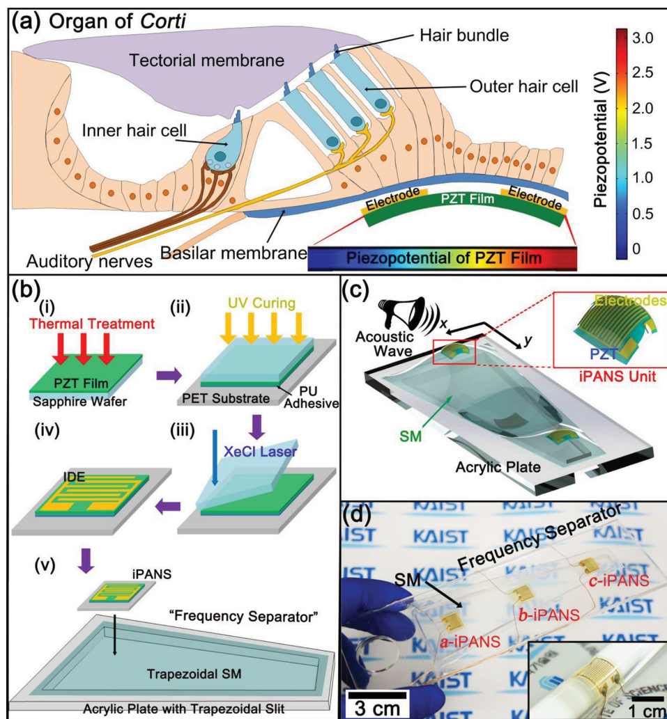
Figure 1. a) Conceptual schematics of organ of Corti in mammalian cochlea. Thin PZT film was placed under BM, and vibrates in the same manner as BM according to sound wave. When a tensile stress applied parallel to the surface of PZT film, the PZT film was bent upwards with a height of 600 nm and generated piezopotential of \approx 3 V. b) Fabrication steps for iPANS i) Coat PZT film on a sapphire wafer is thermally treated for its crystallization via RTA process. ii) PZT film bonded onto a flexible supporting substrate (PET substrate) with PU adhesive and is cured by UV light. iii) The sapphire wafer is removed from the PZT film with XeCl laser beam via LLO process. iv) Au IDE patterned on the flexible PZT film. v) The flexible iPANS attached onto the frequency separator, which is made up of a trapezoidal SM covering acrylic plate with trapezoidal slit. c) According to acoustic wave, SM vibrated due to resonance; iPANS is mechanically deformed in response to vibration, resulting in converting into electricity. d) Photograph of the frequency separator with iPANS. The inset shows a single iPANS unit attached to a glass rod with a radius of curvature of 1.0 cm.
