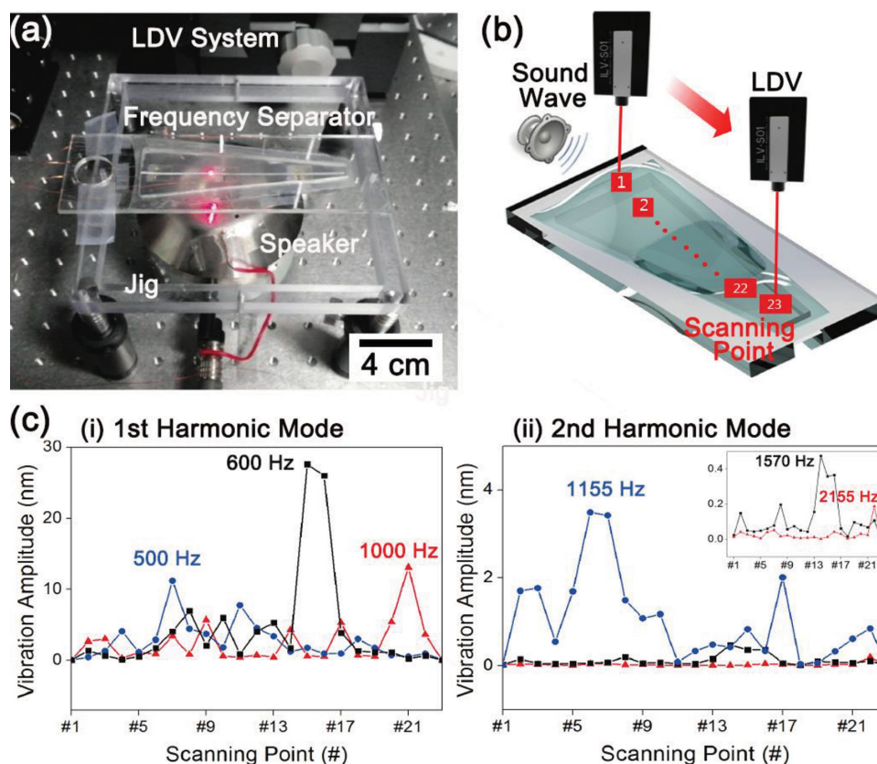
Figure 4. a) Experiment setup with several apparatuses for measuring the vibration amplitude of iPANS in response to the sound coming from a speaker. b) LDV system scanned point by point over all longitudinal-axis of SM. Total 23 scanning points were observed. c) Peak of vibration over all scanning points in i) 1 st harmonic mode and ii) 2 nd harmonic mode. Most of vibration amplitude in 2 nd harmonic mode was under 5 nm, which is much smaller than that of 1 st harmonic mode.
