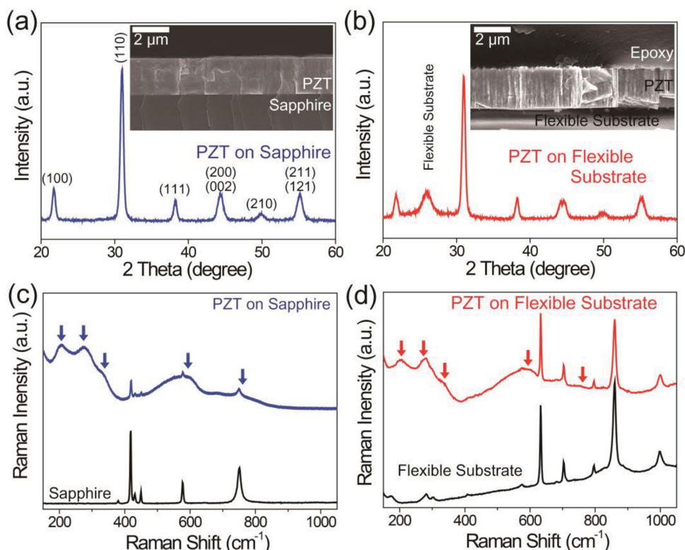
Figure 2. a) XRD analysis result of PZT film on a bulk sapphire wafer before transfer process. The inset shows SEM image of PZT film on the sapphire wafer. b) XRD analysis result of PZT film on a flexible substrate after transfer process. This inset shows SEM image of PZT film on the flexible substrate and covered by SU8 epoxy. c) Raman spectra of PZT film on the sapphire wafer before transfer process. The curves indicated by arrows show the archetypal perovskite PZT phase. d) Raman spectra of PZT film on the flexible substrate after transfer process.
