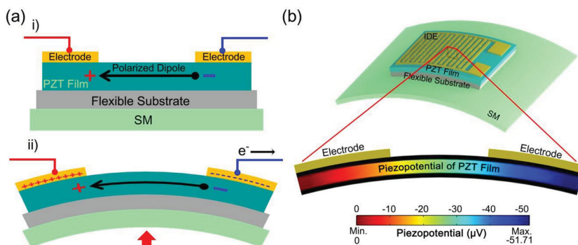
Figure 3. a) Schematics of the working principle in generating piezoelectricity of iPANS unit i) before and ii) after bending deformation. b) Simulated piezopotential distribution inside a PZT film between adjacent electrodes. The dimension of simulated model corresponds to that of actual model.
